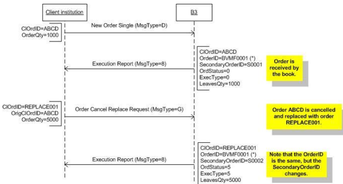
Figure 11 - Order modification scenario - OrderID is kept for modified order.
