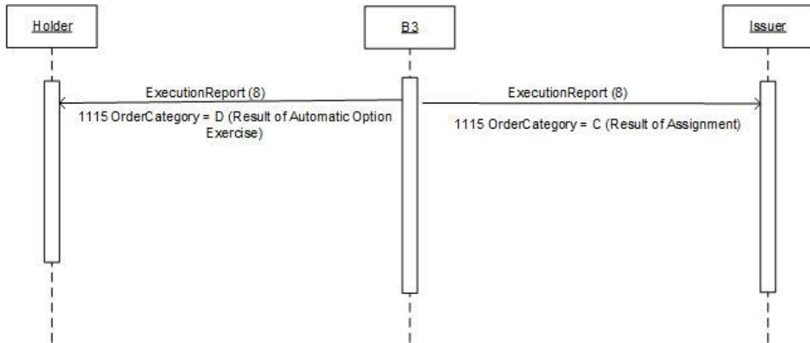
Figure 32 – Trade Notification Due Automatic Exercise Execution scenario
