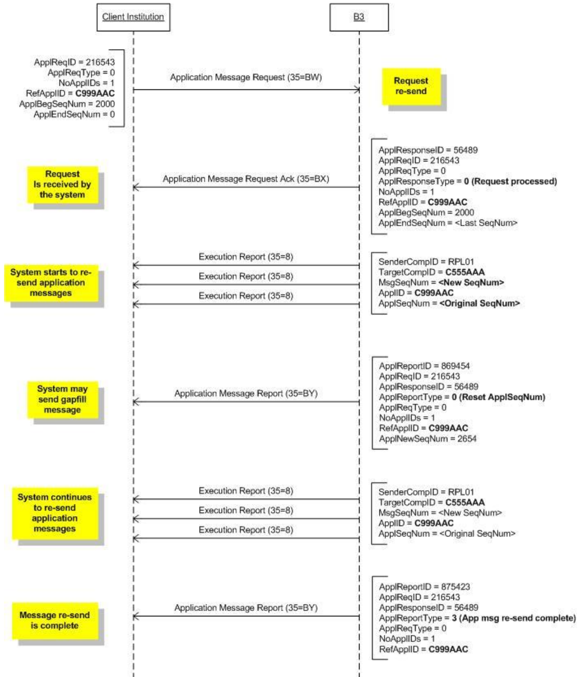
Figure 53 - Message Re-send
