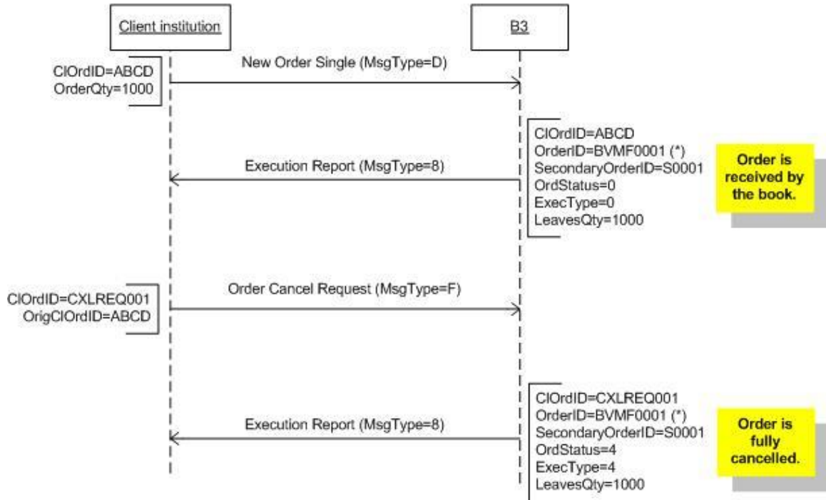
Figure 8 - Order cancellation using CIOrdID
