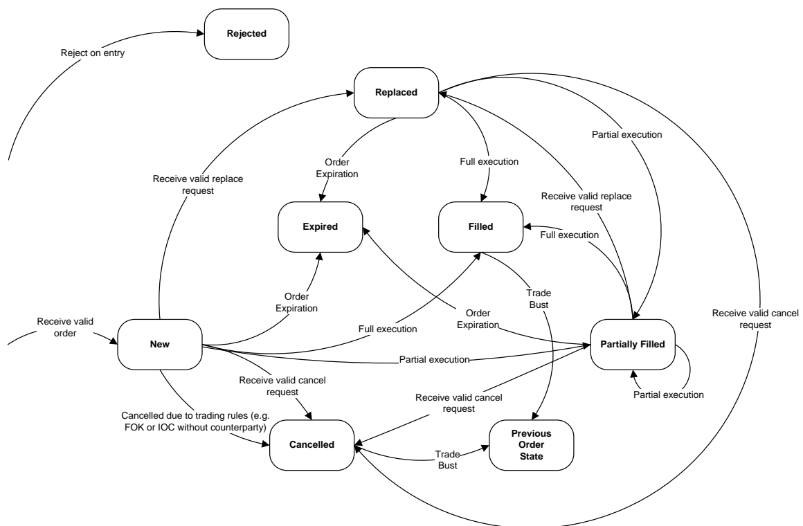
Figure 3 - Order State Transitions
