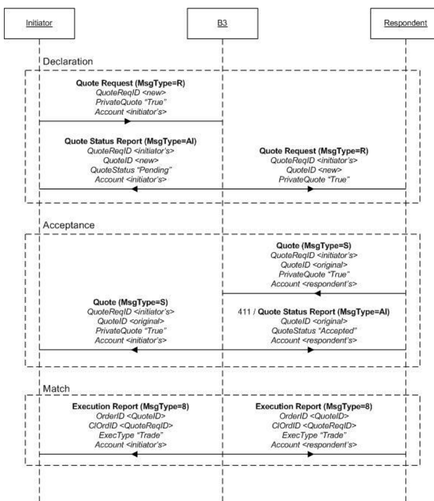
Figure 35 - Forward Matching scenario
