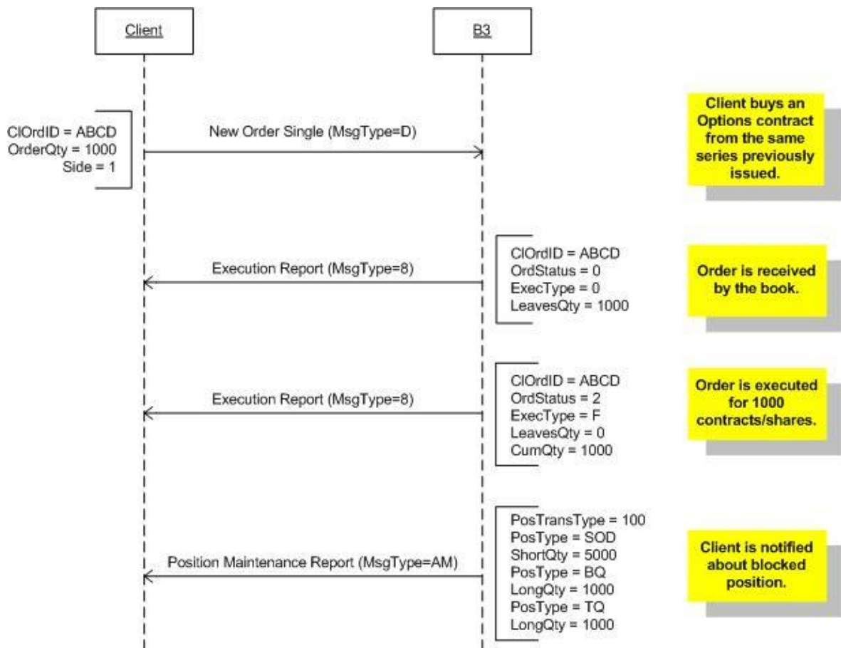
Figure 16 - Automatic Blocking scenario
