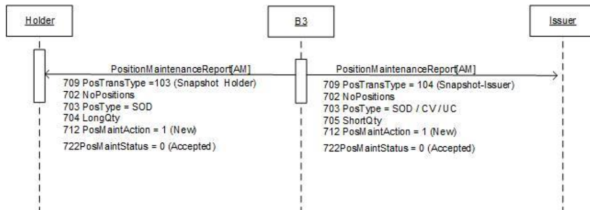
Figure 20 – Incremental Position Snapshot scenario
