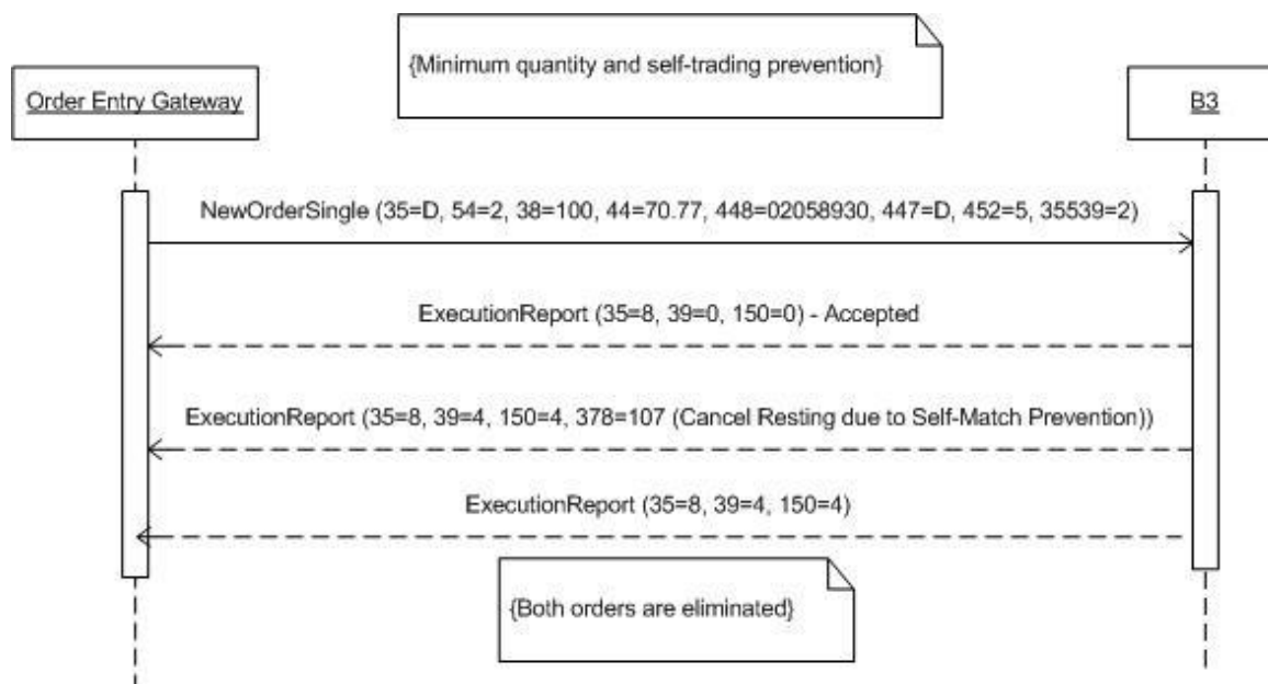
Figure 51 – Minimum quantity and self-Trading prevention
