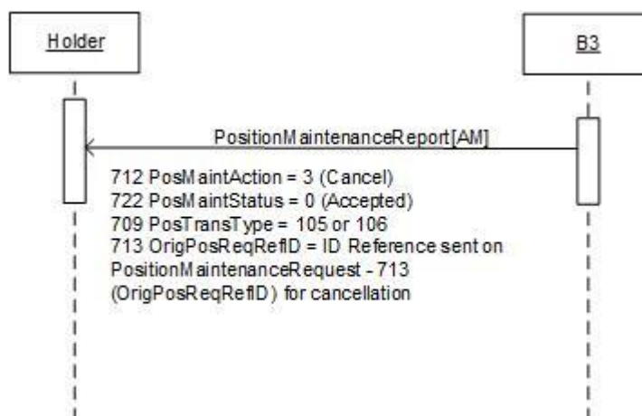
Figure 28 – Contrary Exercise Cancel Response - Acceptance by the Exchange scenario
