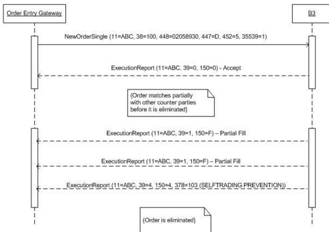
Figure 52 - Self-Trading prevention and partial fills
