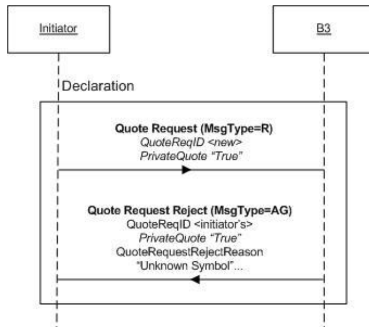
Figure 45 - Cross Forward Rejection scenario
