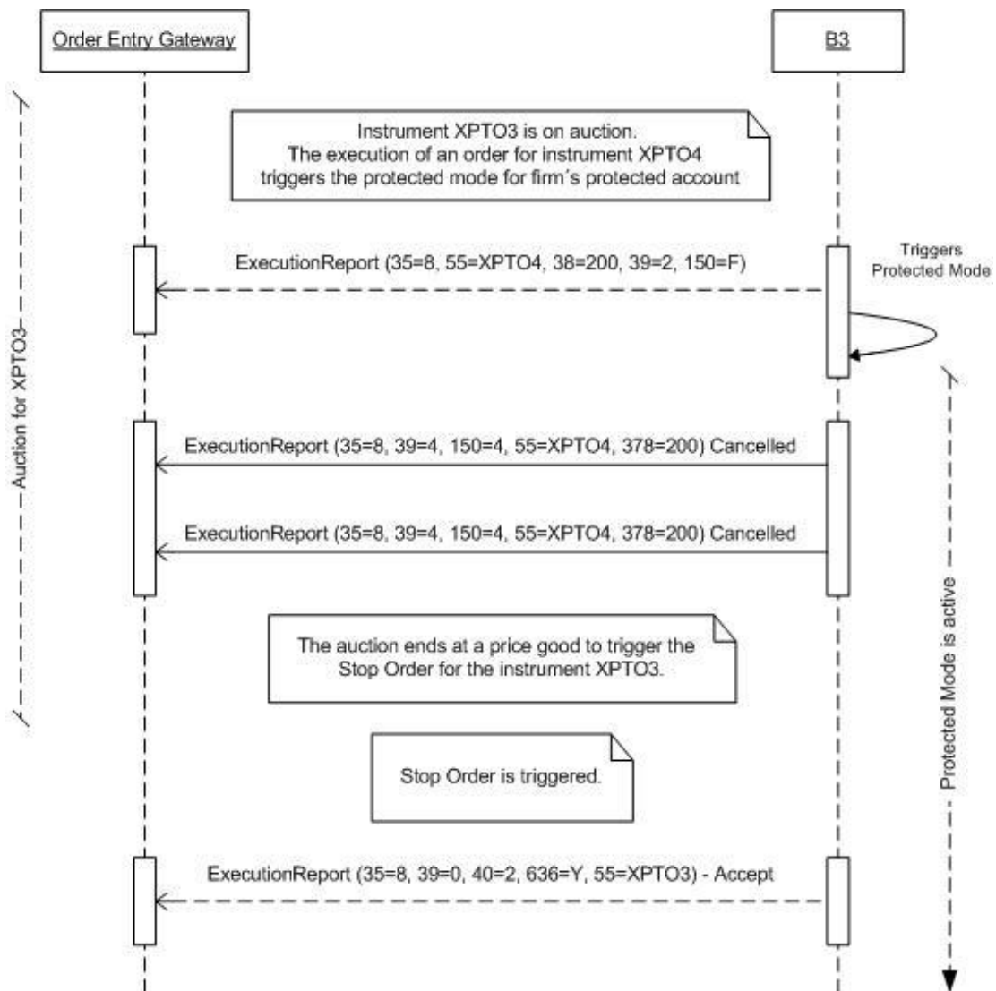
Figure 66 - Stop Order not cancelled at Protection Mode activation
