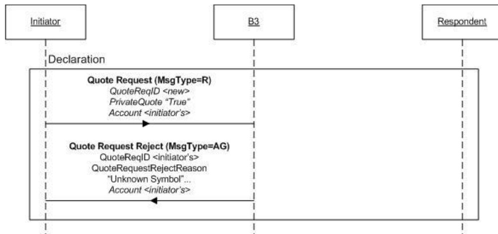
Figure 18 - Forward Declaration Rejection scenario
