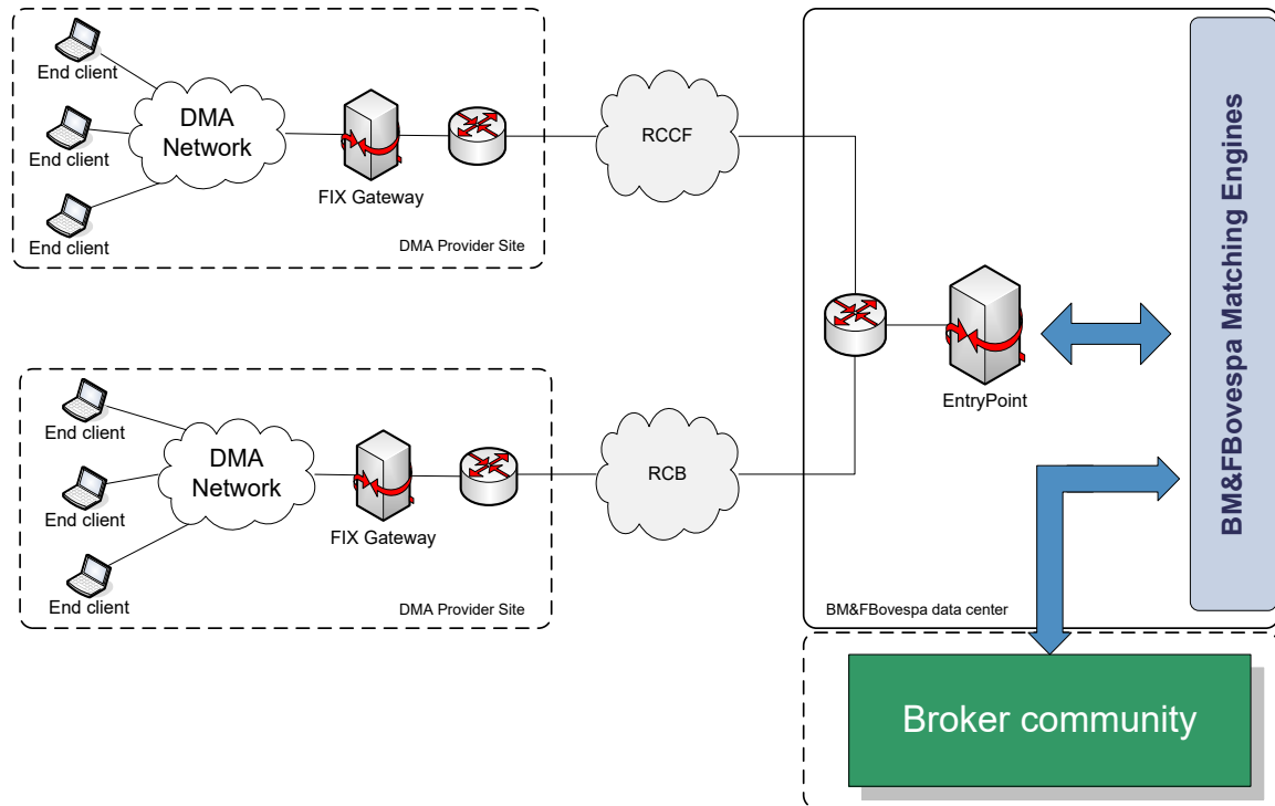
Figure 1 - B3 DMA providers' network setup
