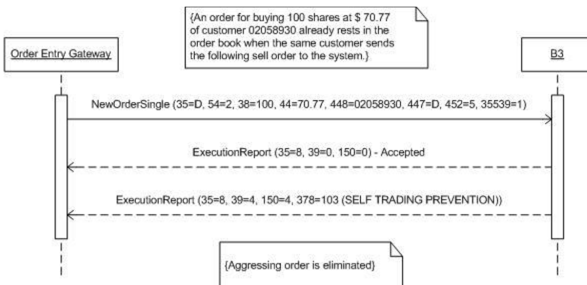
Figure 48 - Self-Trading prevention on aggressor order
