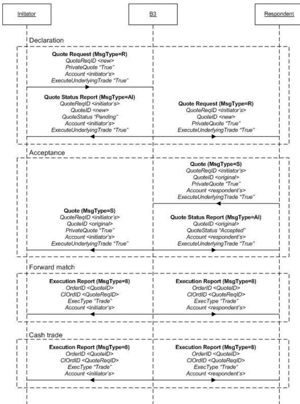
Figure 46 - Forward + Cash scenario
