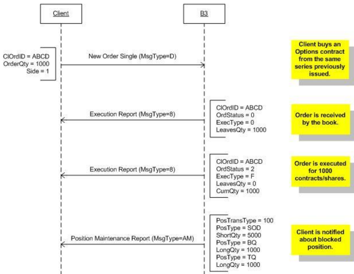
Figure 16 - Automatic Blocking scenario
