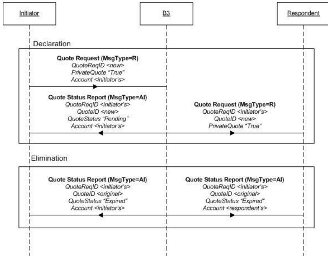
Figure 42 - Forward Expiration scenario
