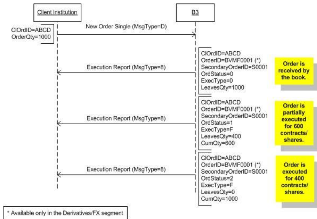
Figure 7 - Order Entry with partial and total fill
