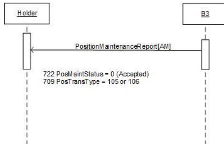
Figure 24 – Contrary Exercise Response - Acceptance by the Exchange scenario
