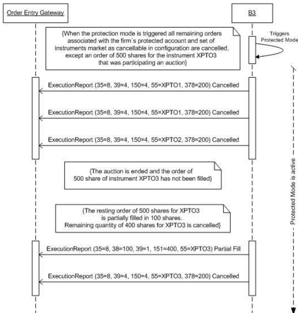
Figure 64 - Order Partially Filled and Remaining Quantity Cancelled
