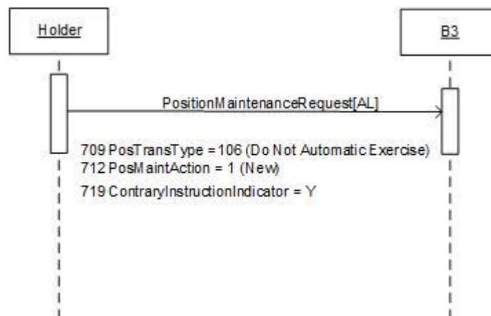
Figure 23 – Request to Abandon Exercise of ITM positions scenario
