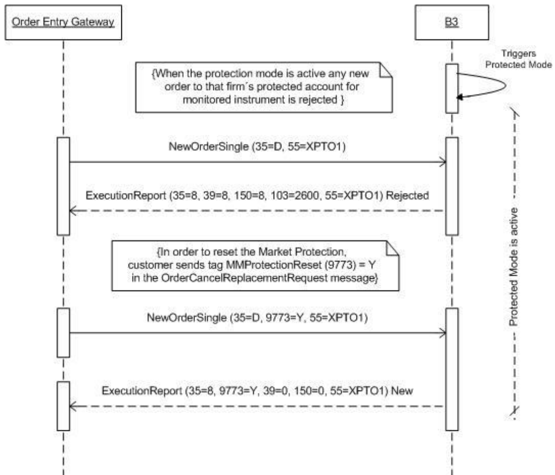
Figure 62 - Resetting Monitoring Mode with Order Cancel Replace Request
