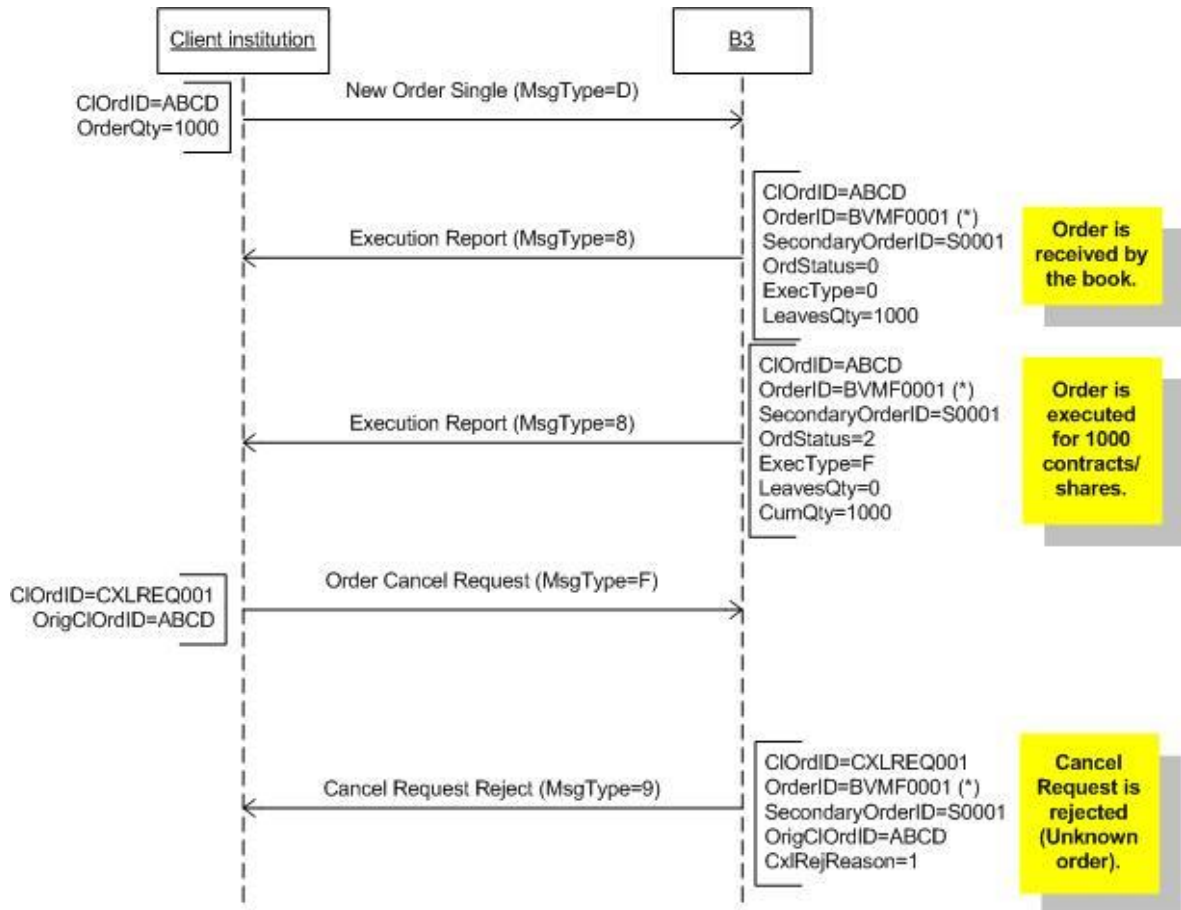
Figure 10 - Attempt to cancel a filled order
