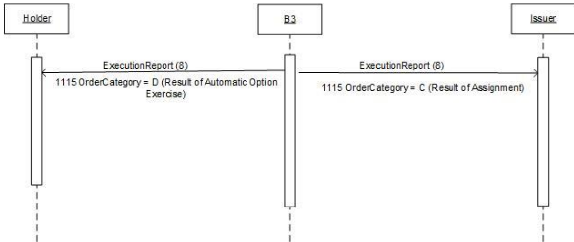
Figure 32 – Trade Notification Due Automatic Exercise Execution scenario
