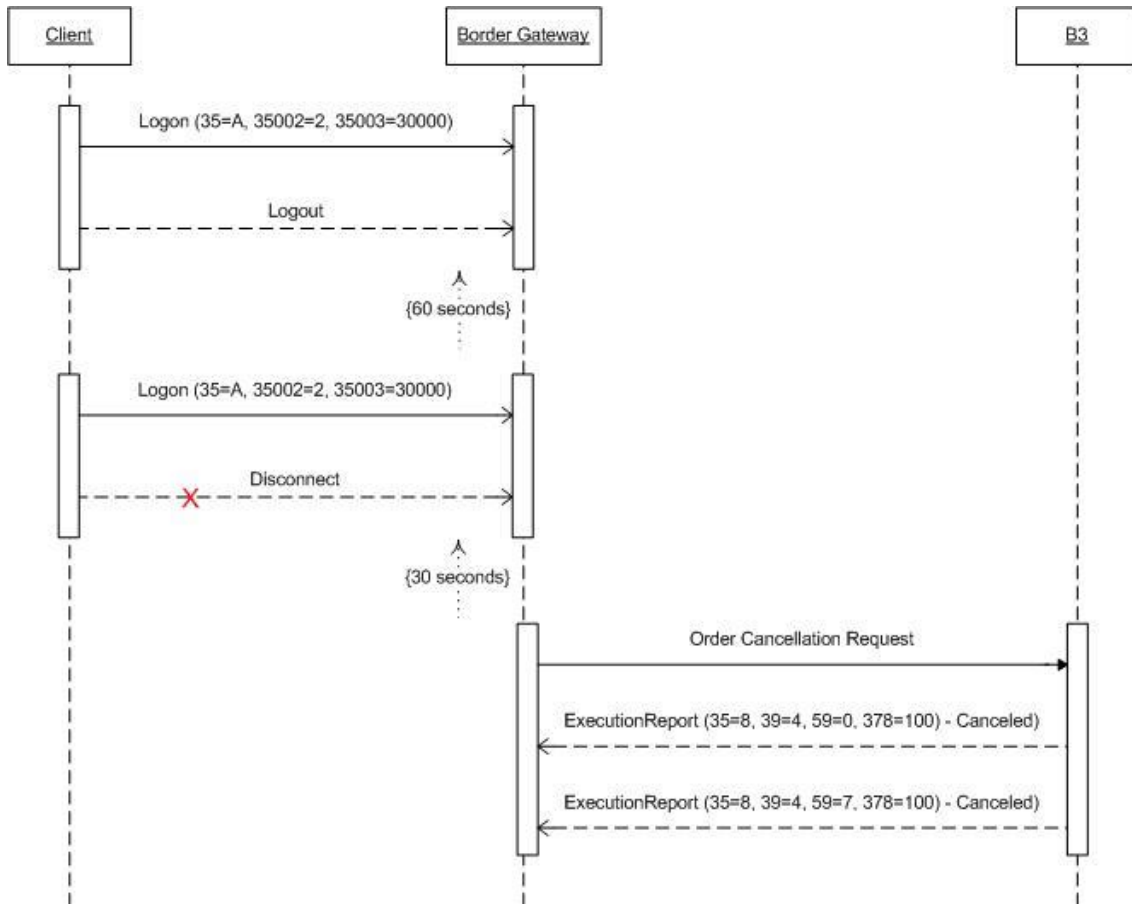
Figure 14 - Cancel On Logout Only
