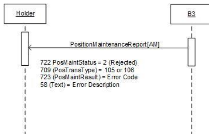
Figure 25 -- Contrary Exercise Response - Rejection by the Exchange scenario
