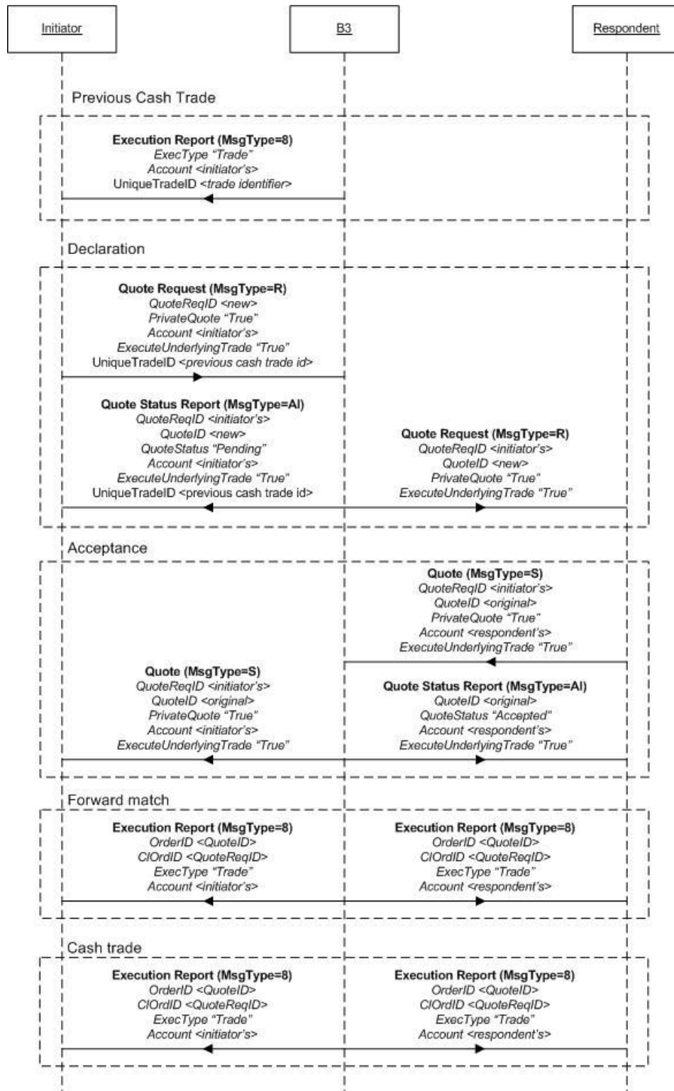
Figure 47 - Forward + Registered Cash scenario
