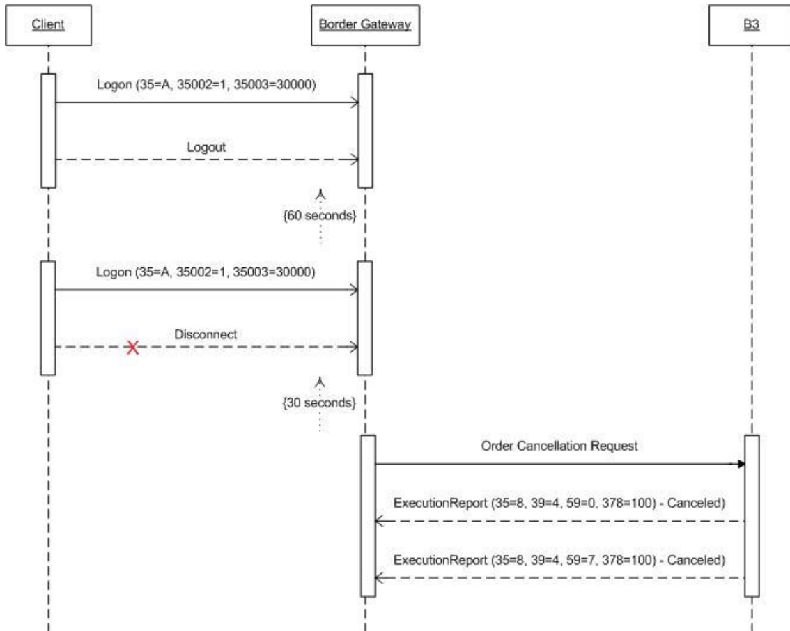
Figure 13 - Cancel On Disconnect Only
