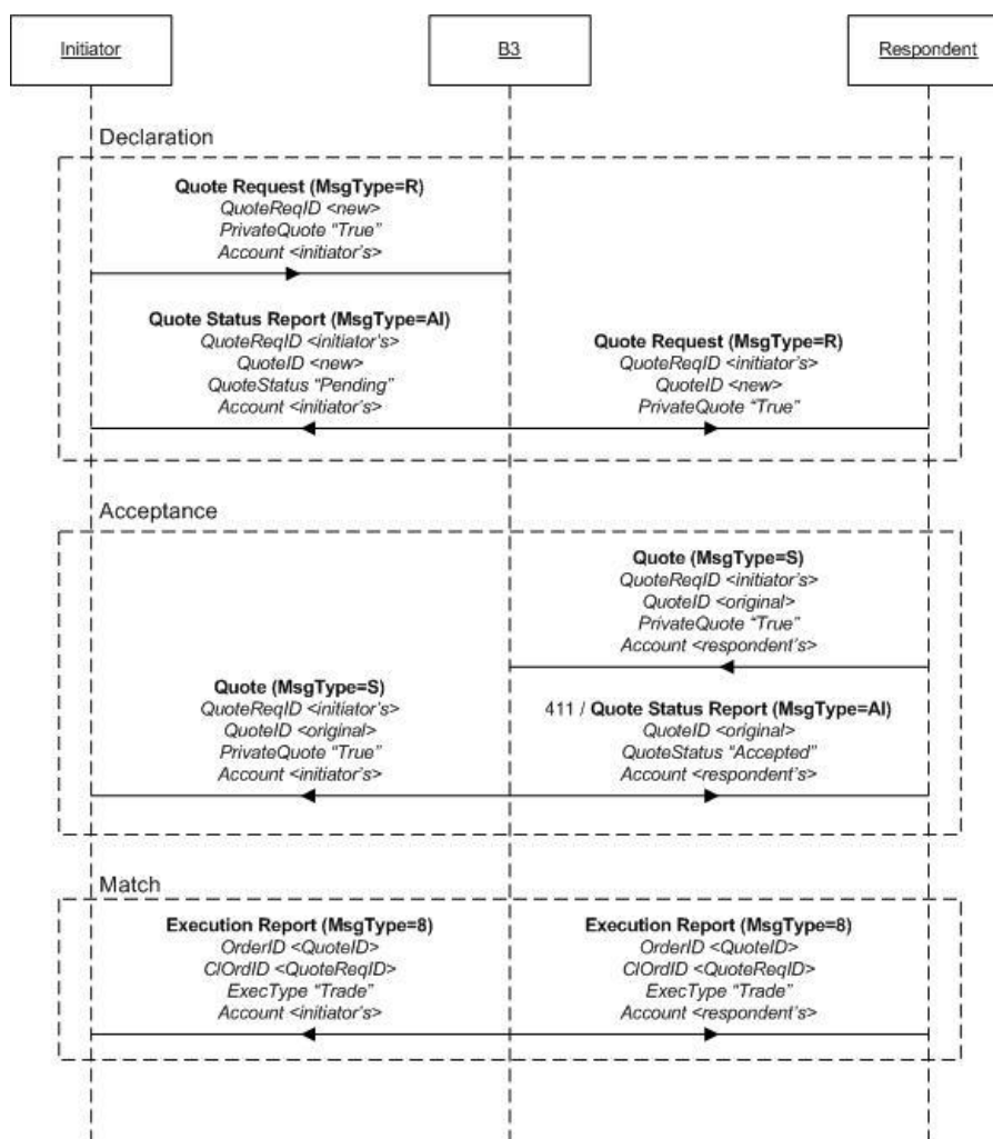
Figure 35 - Forward Matching scenario
