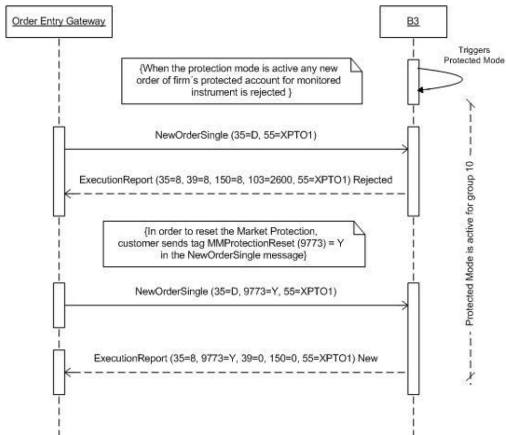
Figure 61 - Resetting Monitoring Mode with New Order Single
