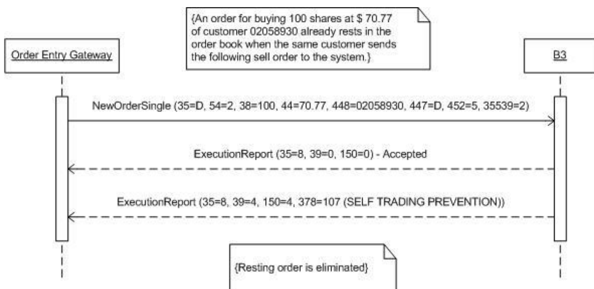
Figure 49 - Self-Trading prevention on resting order
