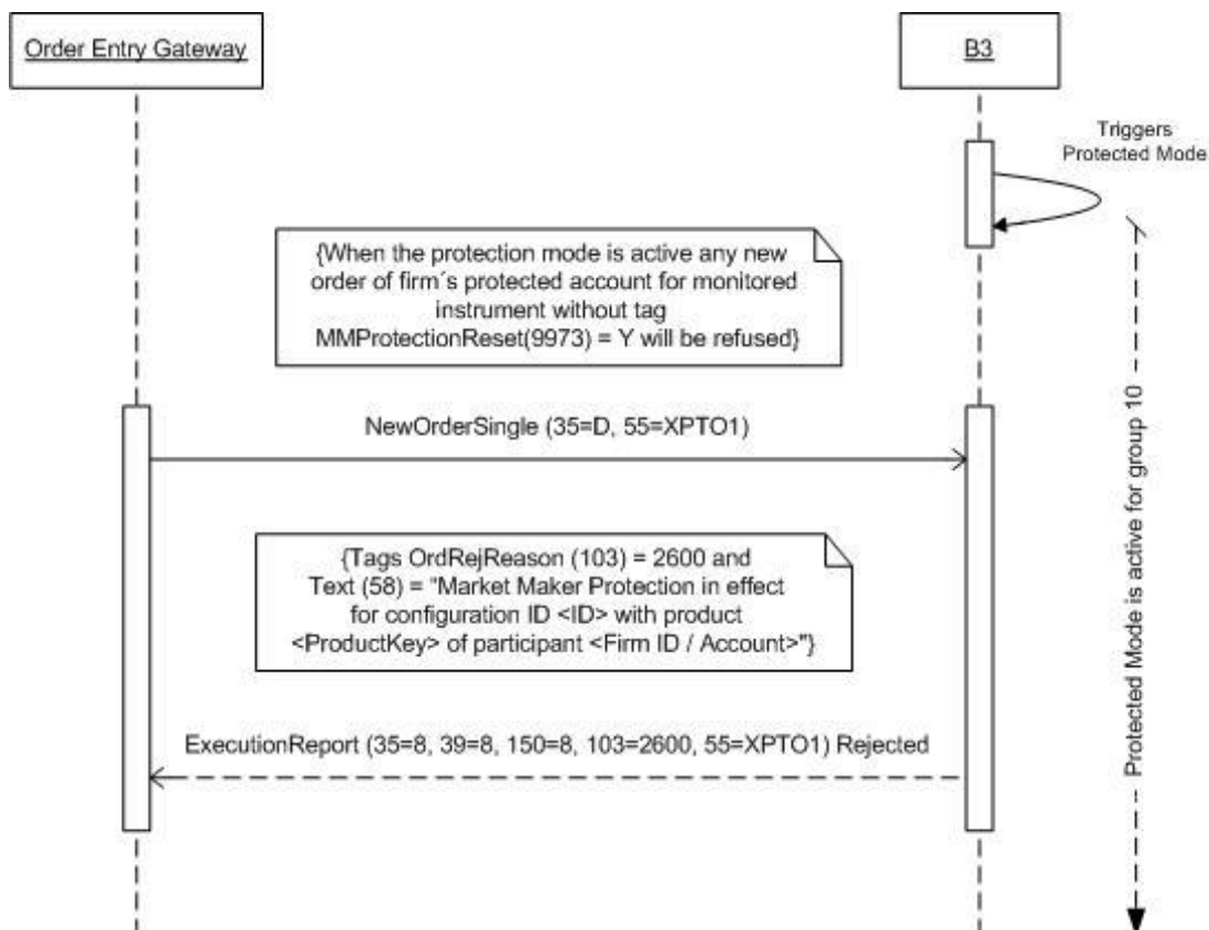
Figure 60 – During Protected Mode New Orders are Rejected
