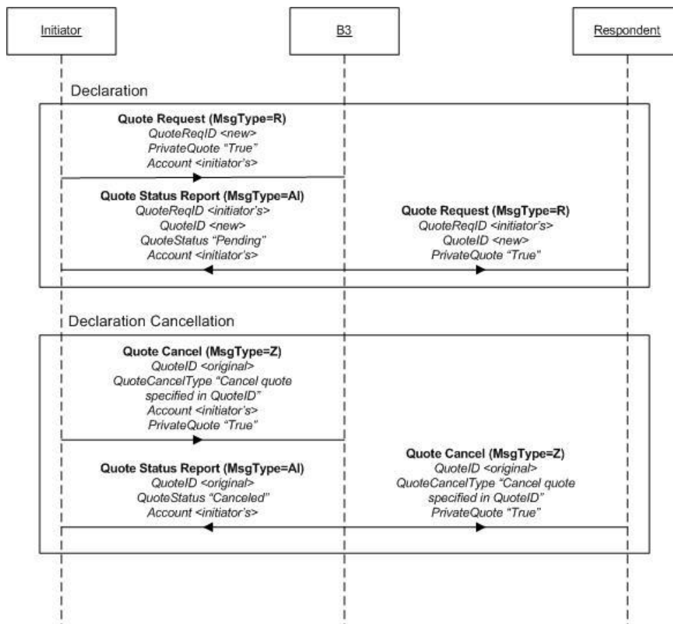
Figure 38 - Forward Declaration Cancellation scenario
