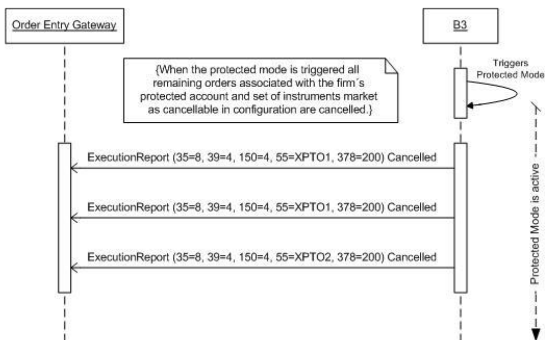
Figure 59 – Remaining Orders are Cancelled when Protection Mode is triggered
