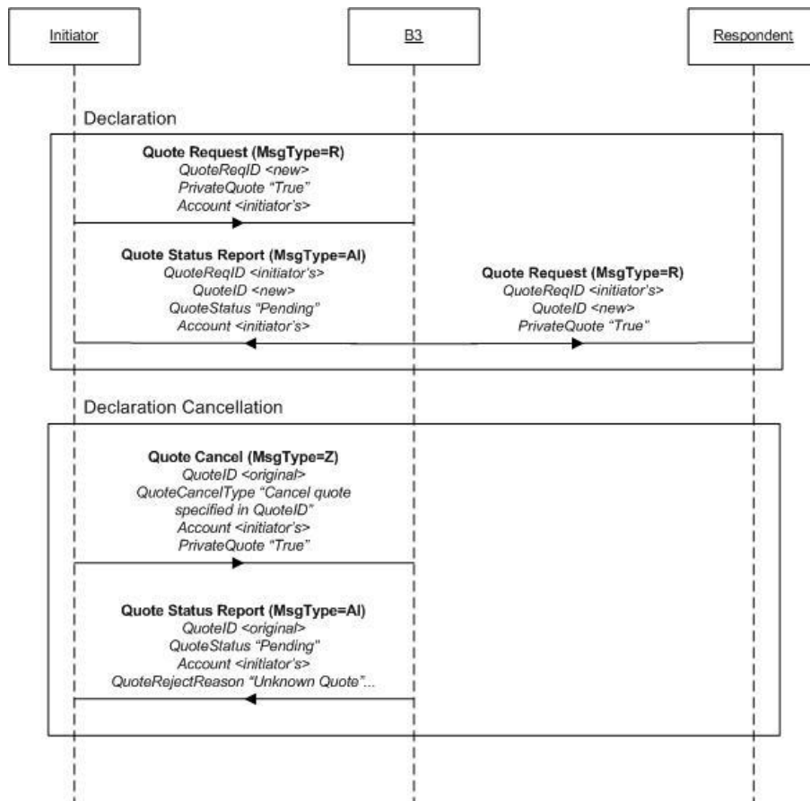
Figure 39 - Forward Declaration Cancellation Rejection scenario
