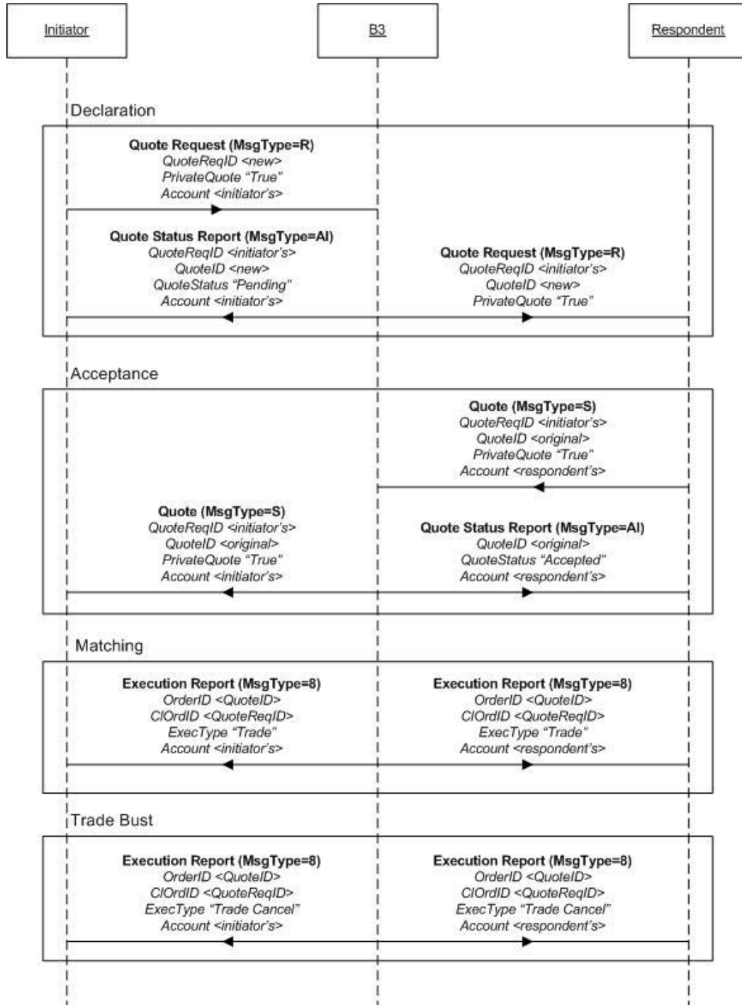
Figure 43 - Forward Trade Bust scenario
