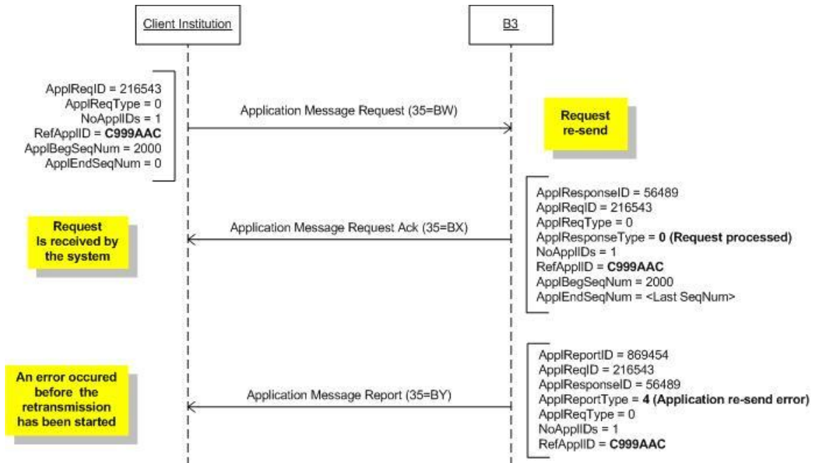
Figure 58 - Error during re-sending
