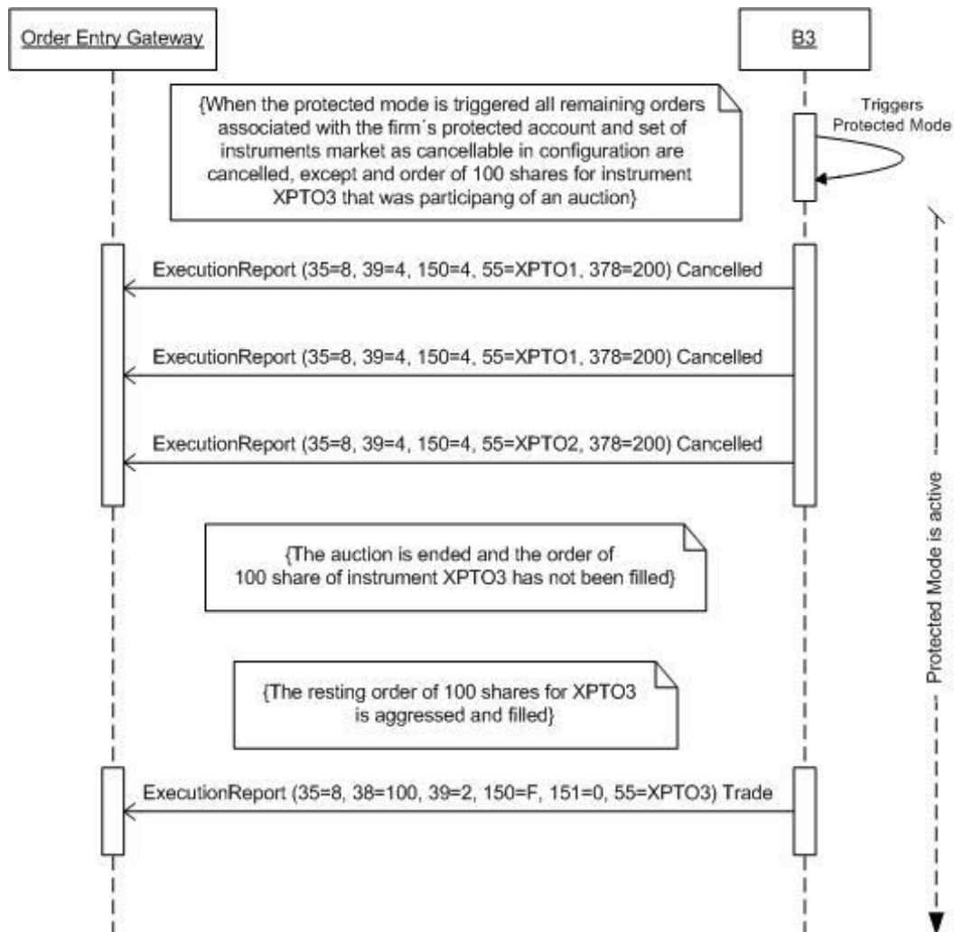
Figure 63 - Order Filled During the Protected Mode
