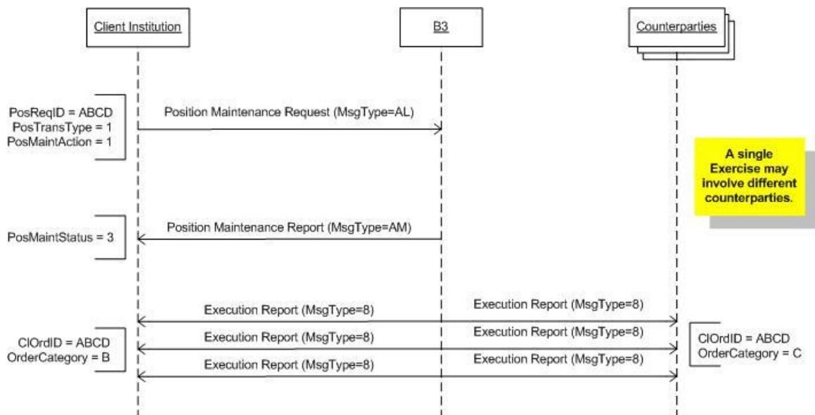
Figure 15 - Option exercise scenario.
