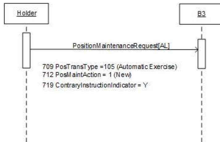
Figure 22 – Request to Exercise ATM or OTM positions scenario
