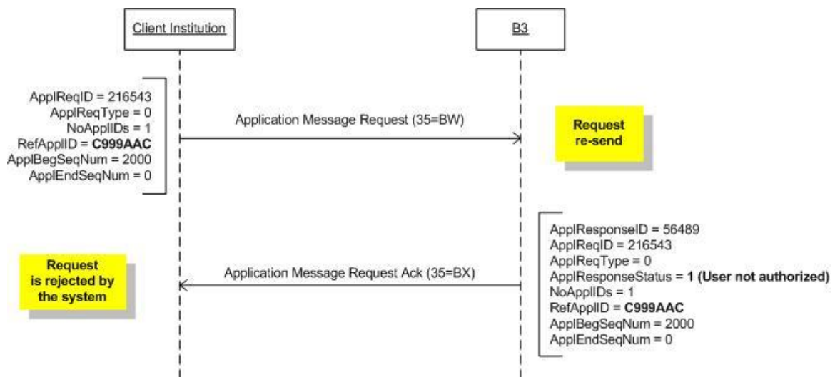
Figure 54 - User not authorized
