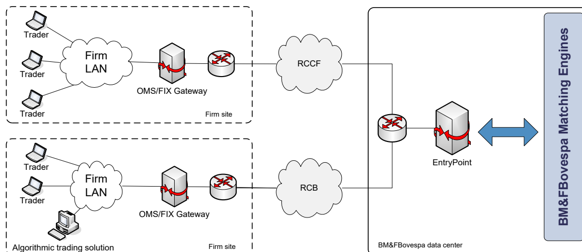
Figure 2 - B3-brokerage firms/banks network setup
