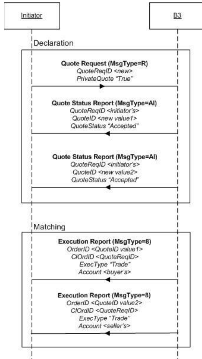
Figure 44 - Cross Forward scenario
