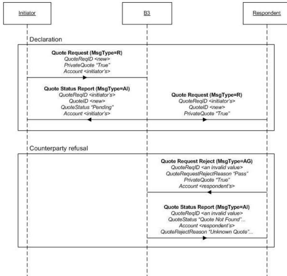
Figure 201 - Forward Counterparty Refusal Rejection scenario
