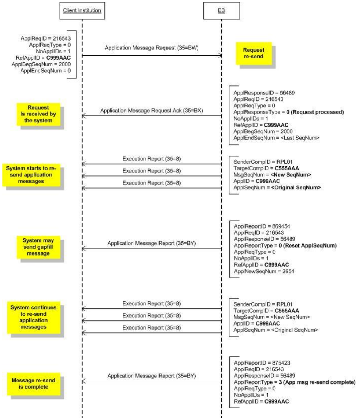
Figure 53 - Message Re-send
