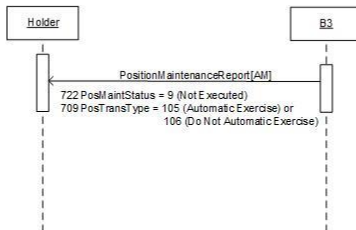
Figure 31 – Contrary Exercise Not Executed scenario
