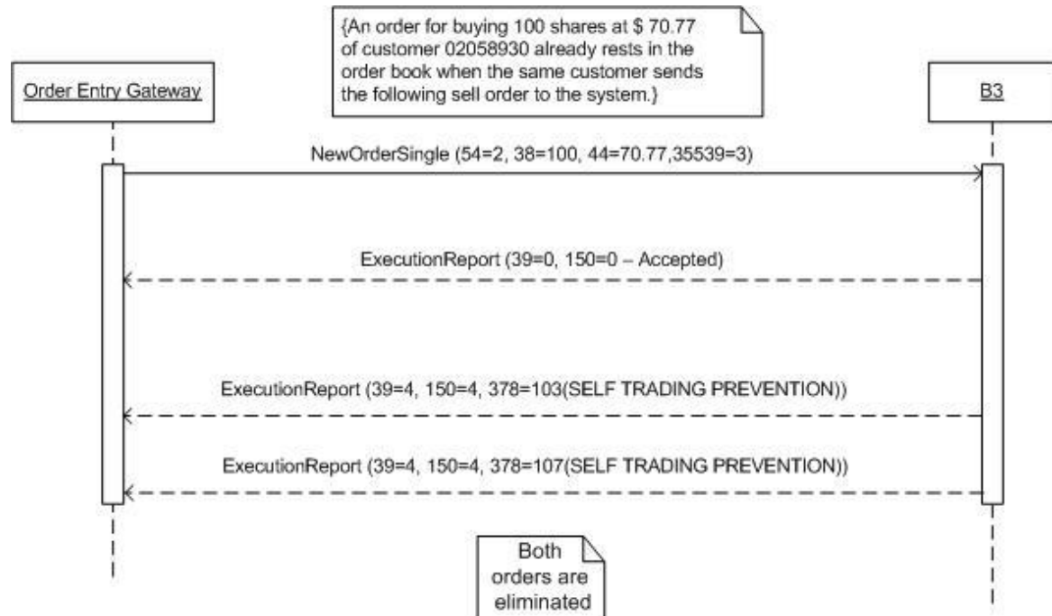
Figure 50 - Self-Trading prevention on both orders
