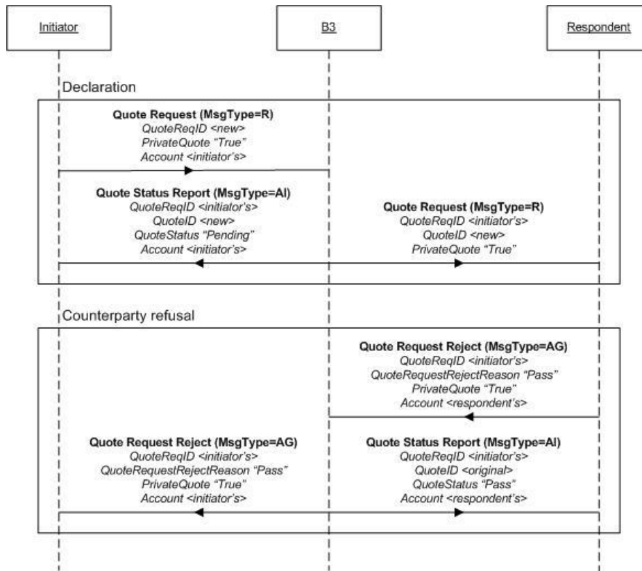
Figure 19 - Forward Counterparty Refusal scenario
