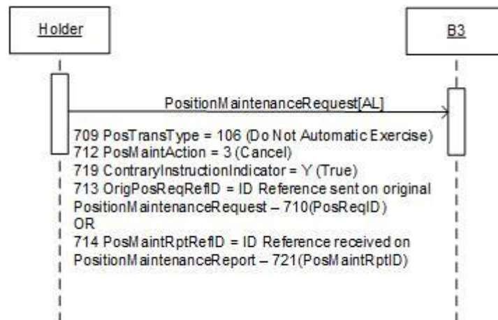
Figure 27 – Cancel of a Request to abandon Exercise of ITM positions scenario
