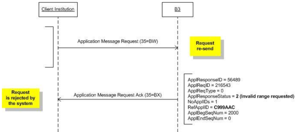
Figure 55 - Invalid range requested
