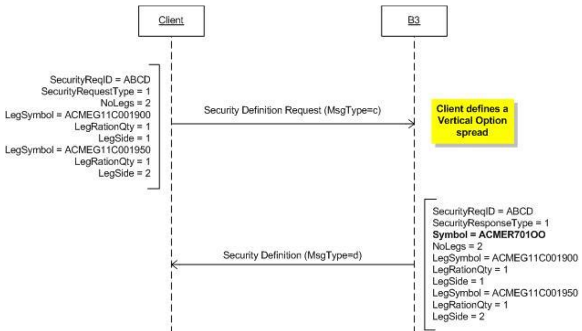
Figure 33 - User-Defined Spread creation scenario
