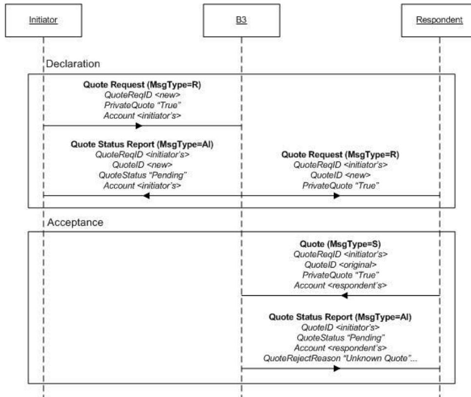
Figure 37 - Forward Acceptance Rejection scenario
