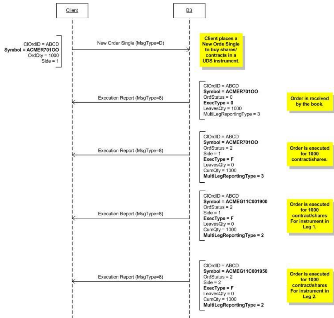
Figure 17 - User-Defined Spread Execution Reports scenario
