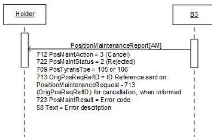
Figure 29 – Contrary Exercise Cancel Response - Rejection by the Exchange scenario
