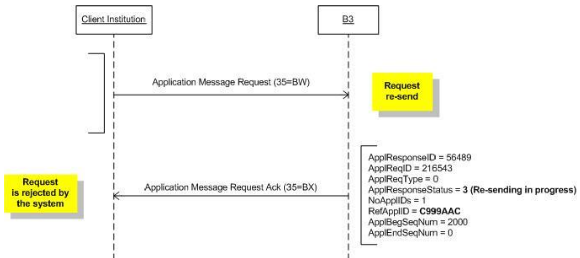
Figure 56 - Re-send already in progress
