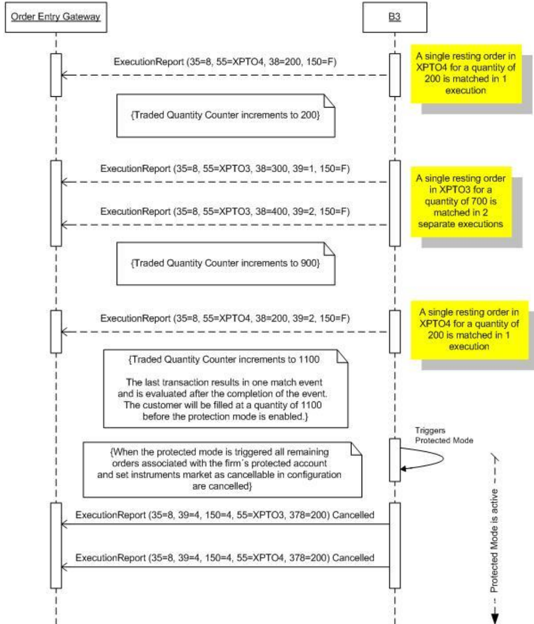
Figure 65 - Order Filled and Protection value Exceeded
