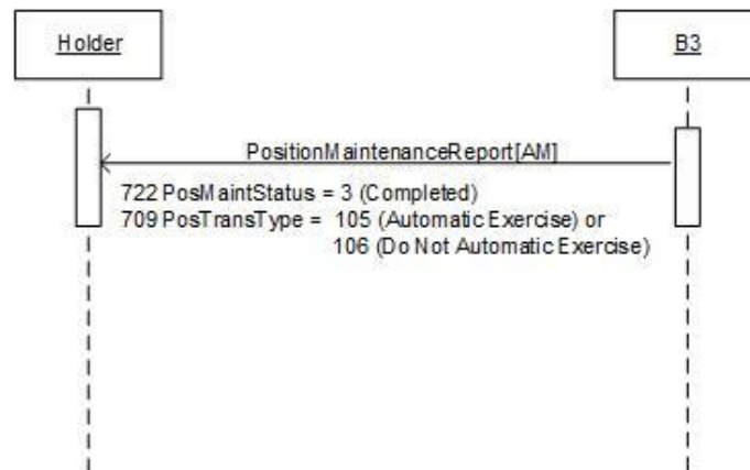
Figure 30 – Contrary Exercise Executed scenario
