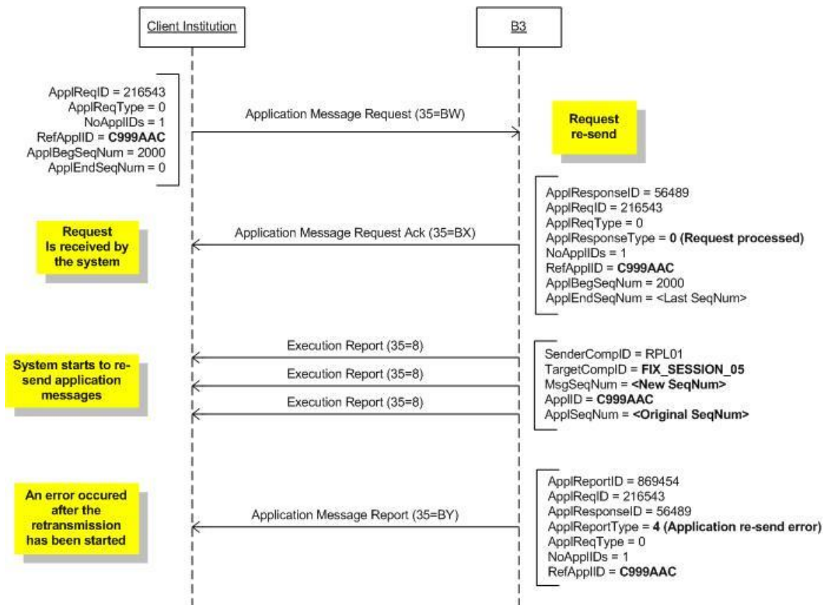
Figure 57 - Error before re-sending
