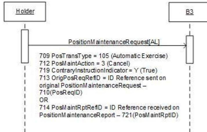
Figure 26 – Cancel of a Request to Exercise ATM and OTM positions scenario
